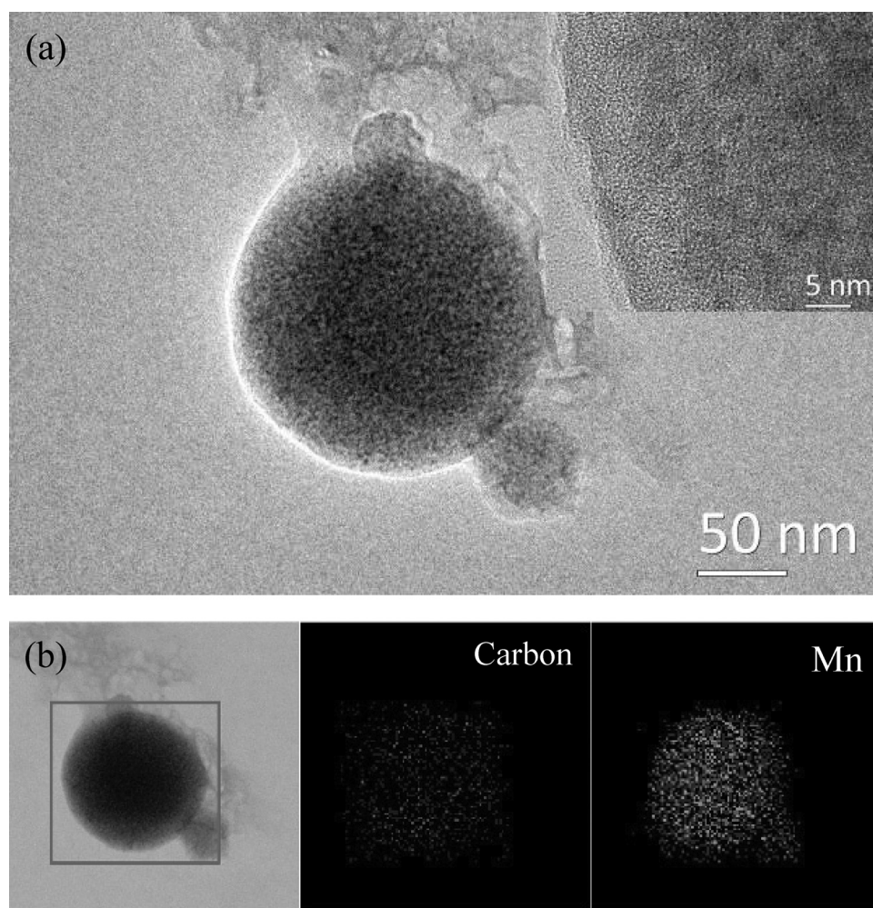
Figure 8. a) TEM images and b) EDS mapping image of distribution of elemental carbon and Mn of the post-cycling amorphous \text{MnO}_x -C nanoparticles.
