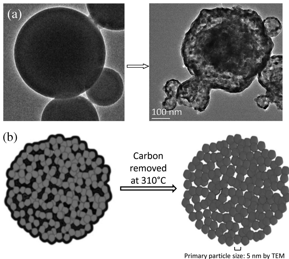
Figure 5. a) TEM image of the amorphous \text{MnO}_x\text{-C} nanoparticles before and after carbon removal at 310 °C, b) Schematic representation of \text{MnO}_x\text{-C} phase structure before and after carbon removal.
